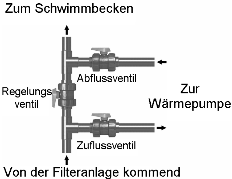
Bypass-Schema
