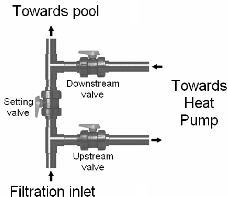
By-pass diagram
