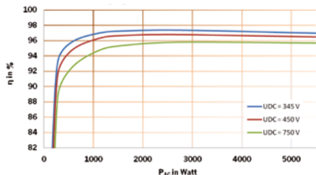
Efficiency curve SOLPLUS 55
